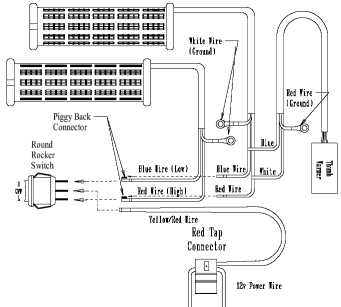
Figure 2. Hand Warmer w/210008 Type Thumb Warmer
